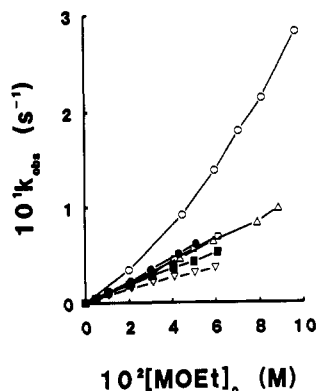
Figure 1. Kinetic data for the reaction of p -nitrophenyl methanesulfonate ( 1 ) with LiOEt ( \nabla ), NaOEt ( \blacksquare ), KOEt ( \Delta ), CsOEt ( \square ), KOEt in the presence of excess 18-crown-6 ( \bullet ), and KOEt in the presence of excess 2.2.2 cryptand ( \circ ) in anhydrous ethanol at 25 °C.
